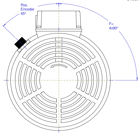
encoder hole
