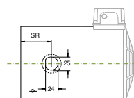
encoder hole
