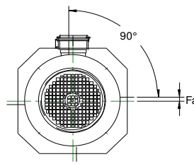
M3AA 112 - 160
