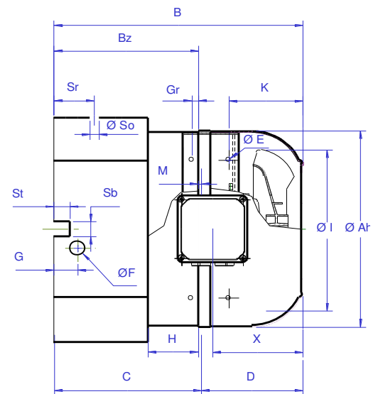
M3AA 112 - 160
