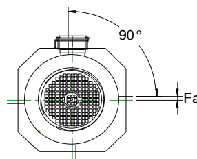
M3AA 112 - 160
