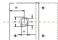
connector / encoder
